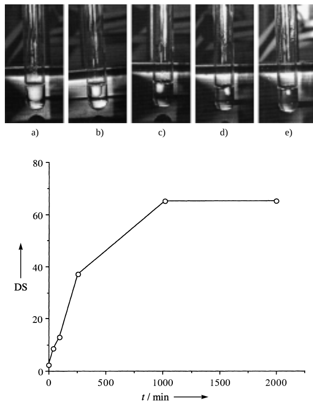
Figure 2. Time dependence of the shrinking of a physically cross-linked gel formed by poly(styrene 19 -NASI 31 -NIPAAm 50 ) at 43 °C at a) 0, b) 40, c) 90, d) 260, and e) 1000 min. The graph presents the dependence of the degree of shrinkage (DS) versus time.
