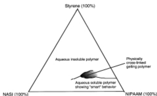
Figure 1. Effect of poly(styrene x -NASI y -NIPAAm z ) composition on the behavior of the polymer in aqueous solutions in response to increasing temperature.
